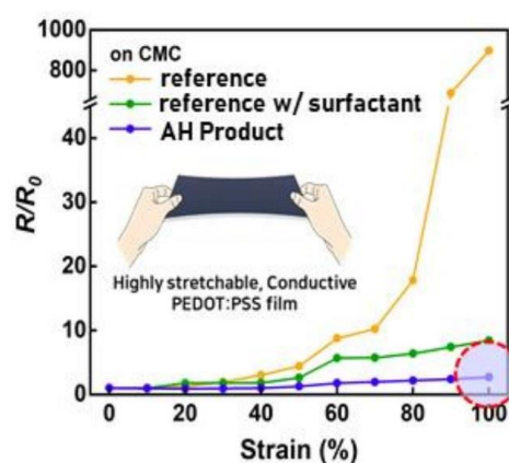
R/R_0 vs. strain on CMC substrate
