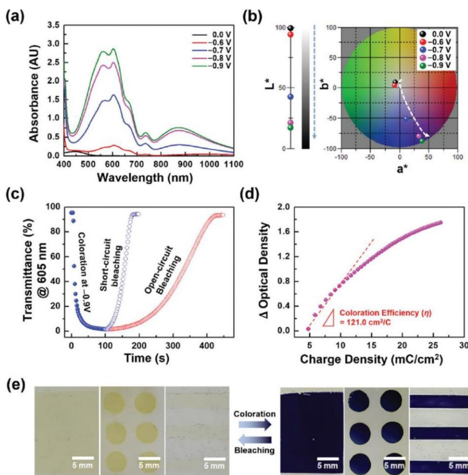
(a) Absorbance and (b) color coordinates at applied voltages; (c) transmittance at 605 nm during coloration and bleaching; (d) coloration efficiency; (e) patterned devices before and after coloration. Ref.: J. Mater. Chem. C 2020, 8, 17045.
