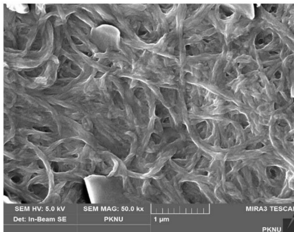
SEM image of AH-PNW (scale bar: 1 μm)
